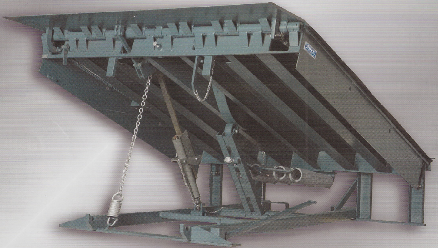
*MP6855 shown with structural C & I beam deck supports and optional weather seal.
