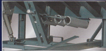
One point adjustable main spring assembly with roller and cam construction.
